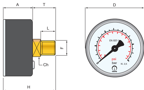
P-Type stem mounted, centre back connection
