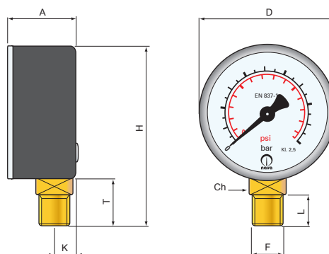
R-Type stem mounted, bottom connection
